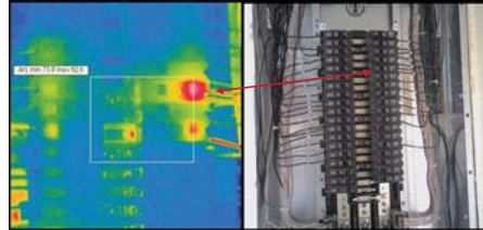
Thermal image reveals overloaded circuit
