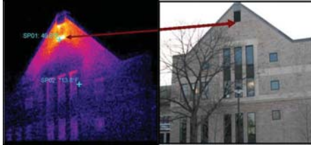
Thermal image reveals significant heat loss
