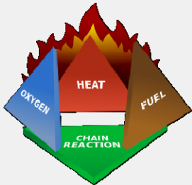
Fire Tetrahedron
